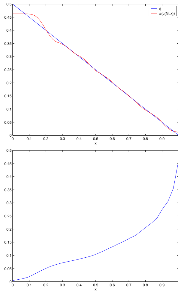
FIGURE 1. Objective function \phi_1 and calculated a(c(x, T)) (left) and computed nonlinear coefficient a(c) (right) for h = \tau = 0.01
