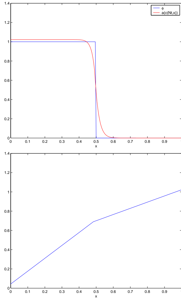
FIGURE 4. Objective function \phi_2 and calculated a(c(x, T)) (left) and computed nonlinear coefficient a(c) (right) for h = \tau = 0.005
