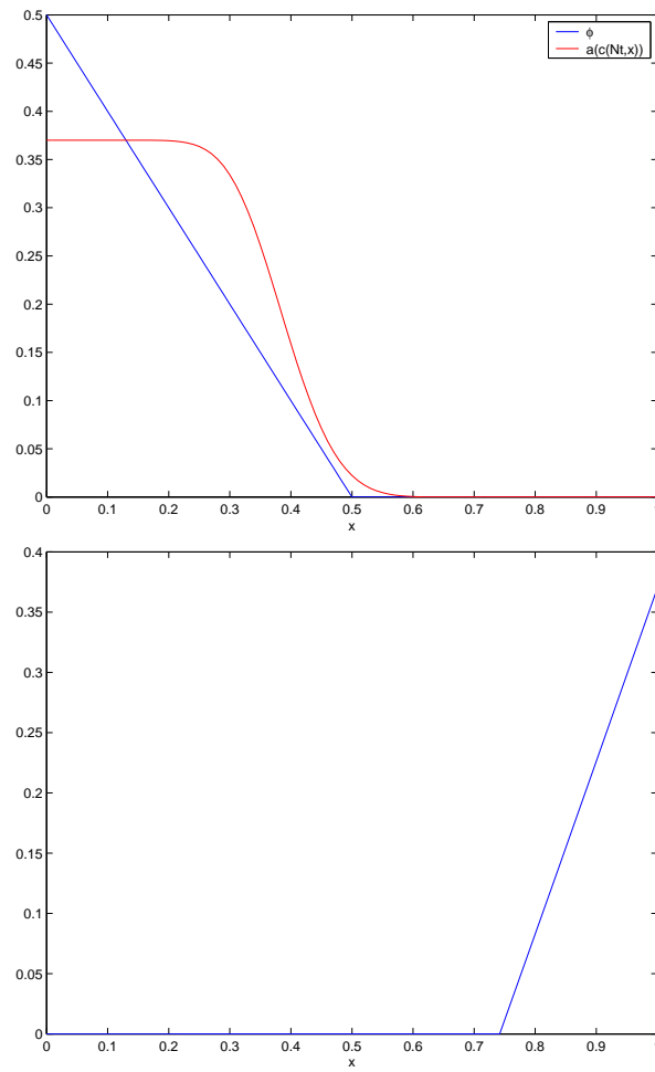
FIGURE 5. Objective function \phi_3 and calculated a(c(x, T)) (left) and computed nonlinear coefficient a(c) (right) for h = \tau = 0.01
